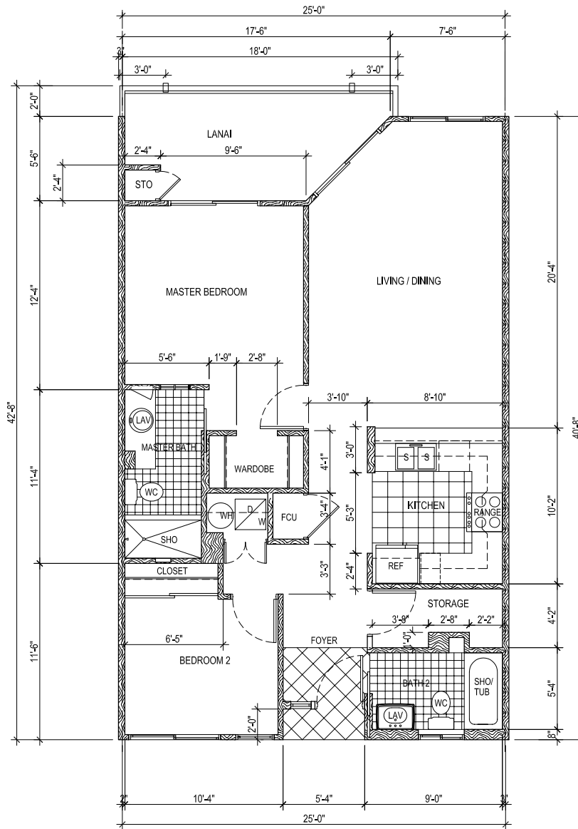
UNIT TYPE "A", TYPE "AR"(REVERSE) TYPICAL FLOOR PLAN
