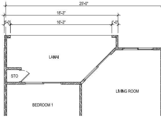
UNIT TYPE "A", TYPE "AR"(REVERSE) PARTIAL GROUND FLOOR PLAN
